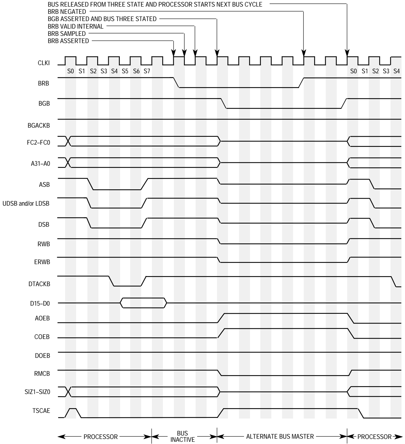
Figure 3-23. 2-Wire Bus Arbitration Timing Diagram—Bus Inactive
