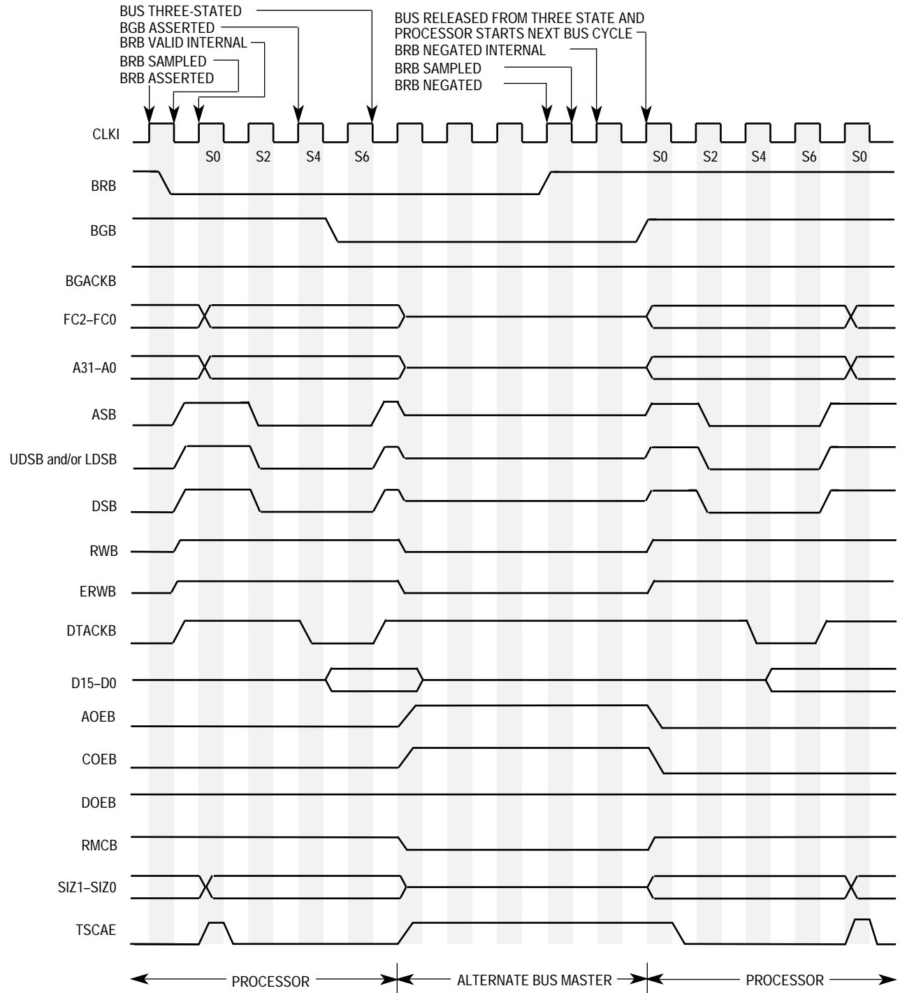
Figure 3-24. 2-Wire Bus Arbitration Timing Diagram—Special Case
